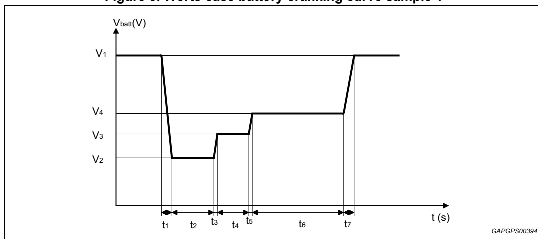
Figure 5. Worts case battery cranking curve sample 1
