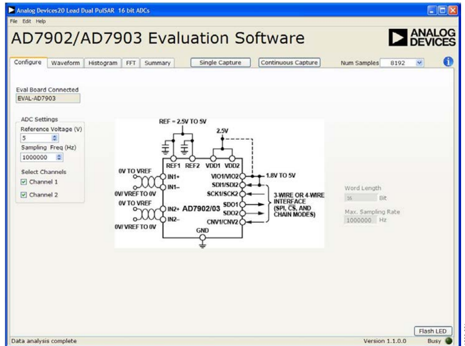
Figure 21. Main Window
