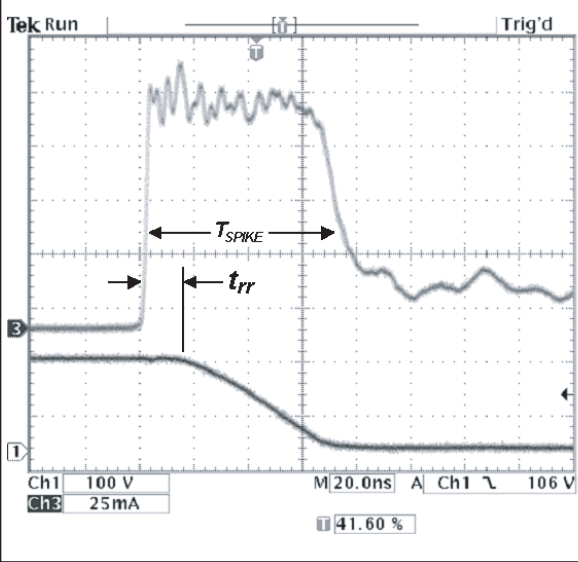
FIGURE 4-6: SWITCH-OFF TRANSITION Ch1:V DRAIN , Ch3: I DRAIN
