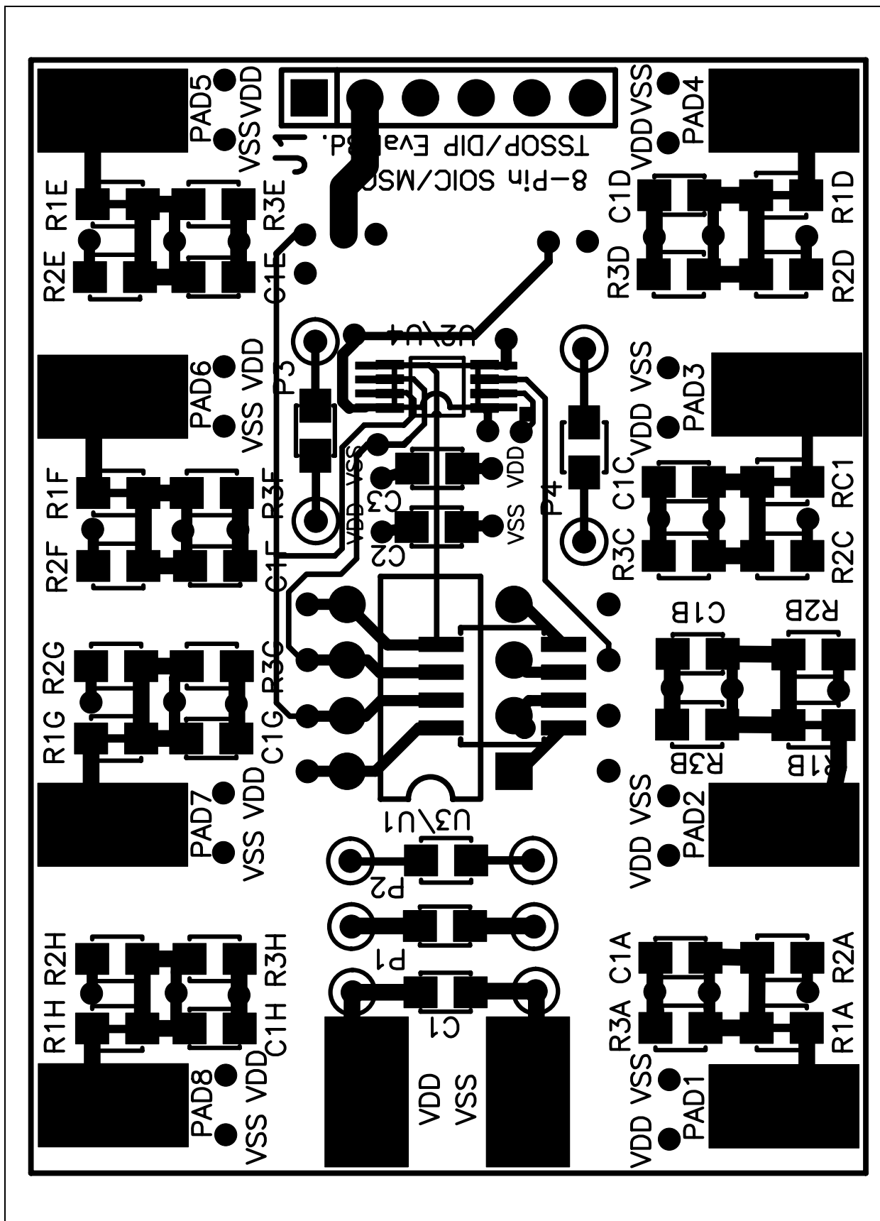
FIGURE A-4: 8-Pin SOIC/MSOP/TSSOP/DIP Evaluation Board Gerber – Top Layer + Silk-Screen.
