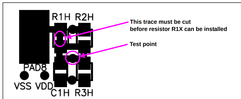
FIGURE 2-4: Test point when resistor R1X is installed.
