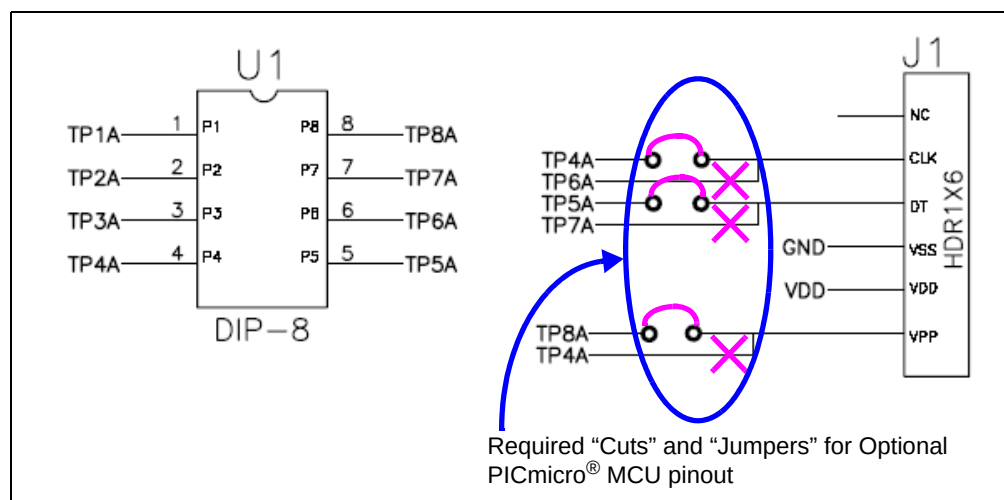
FIGURE 2-5: BFMP Header and Connections
