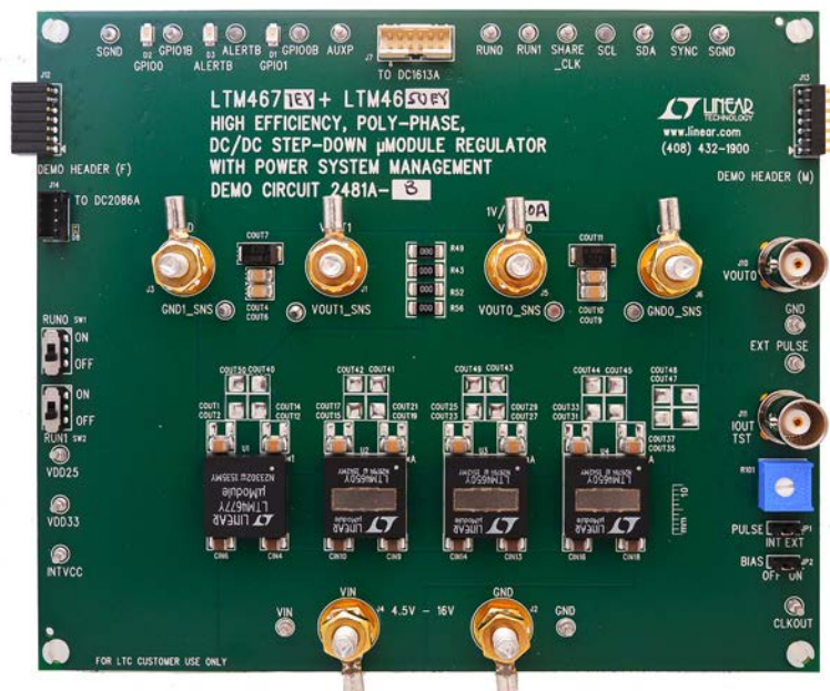
Figure 1. LTM4677 + 3 \times LTM4650; 186A DC2481A-B Demo Circuit
