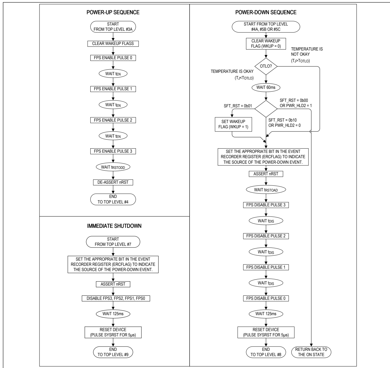
Figure 5. Power-Up/Down Sequence
