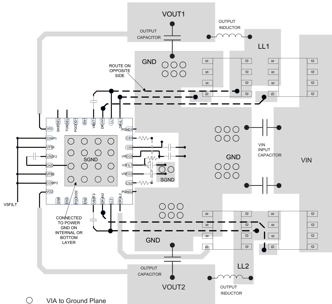
Figure 41. Layout Example
