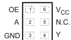
DRY Package 6-Pin SON Transparent Top View
