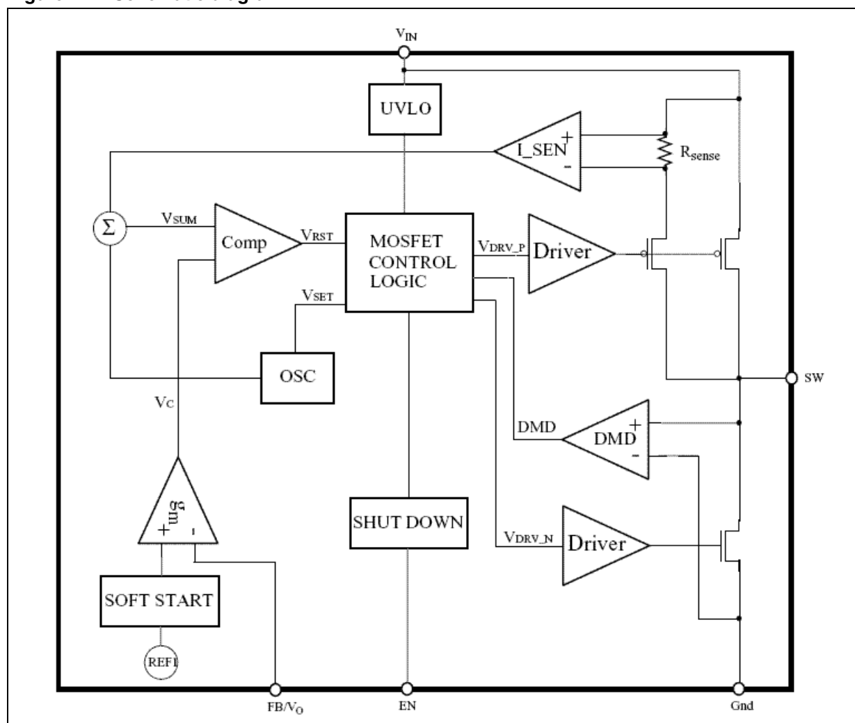
Figure 1. Schematic diagram
