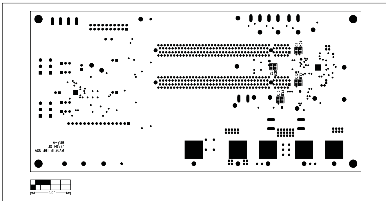
Figure 10. MAX5946L EV Kit Component Placement Guide—Solder Side
