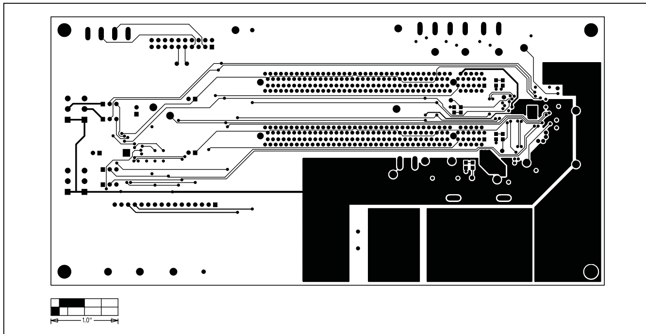
Figure 9. MAX5946L EV Kit PC Board Layout—Solder Side
