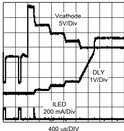
Figure 26. LED String Short Fault and UVP Detection
