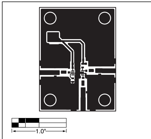
Figure 3. MAX2130 EV Kit PC Board Layout—Component Side
