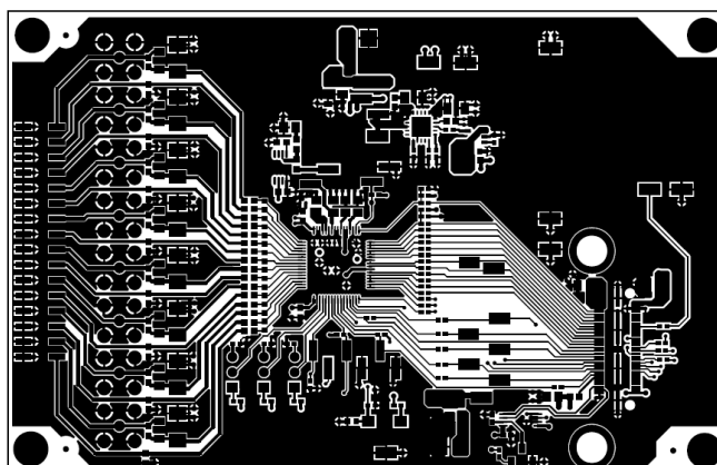
Figure 17. ADS8588S EVM PCB Layer 1: Top Layer
