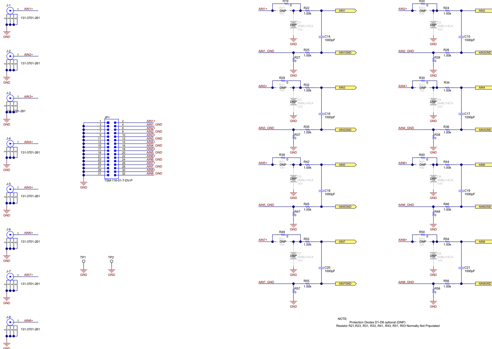
Figure 23. ADS8588EVM-PDK Schematic
