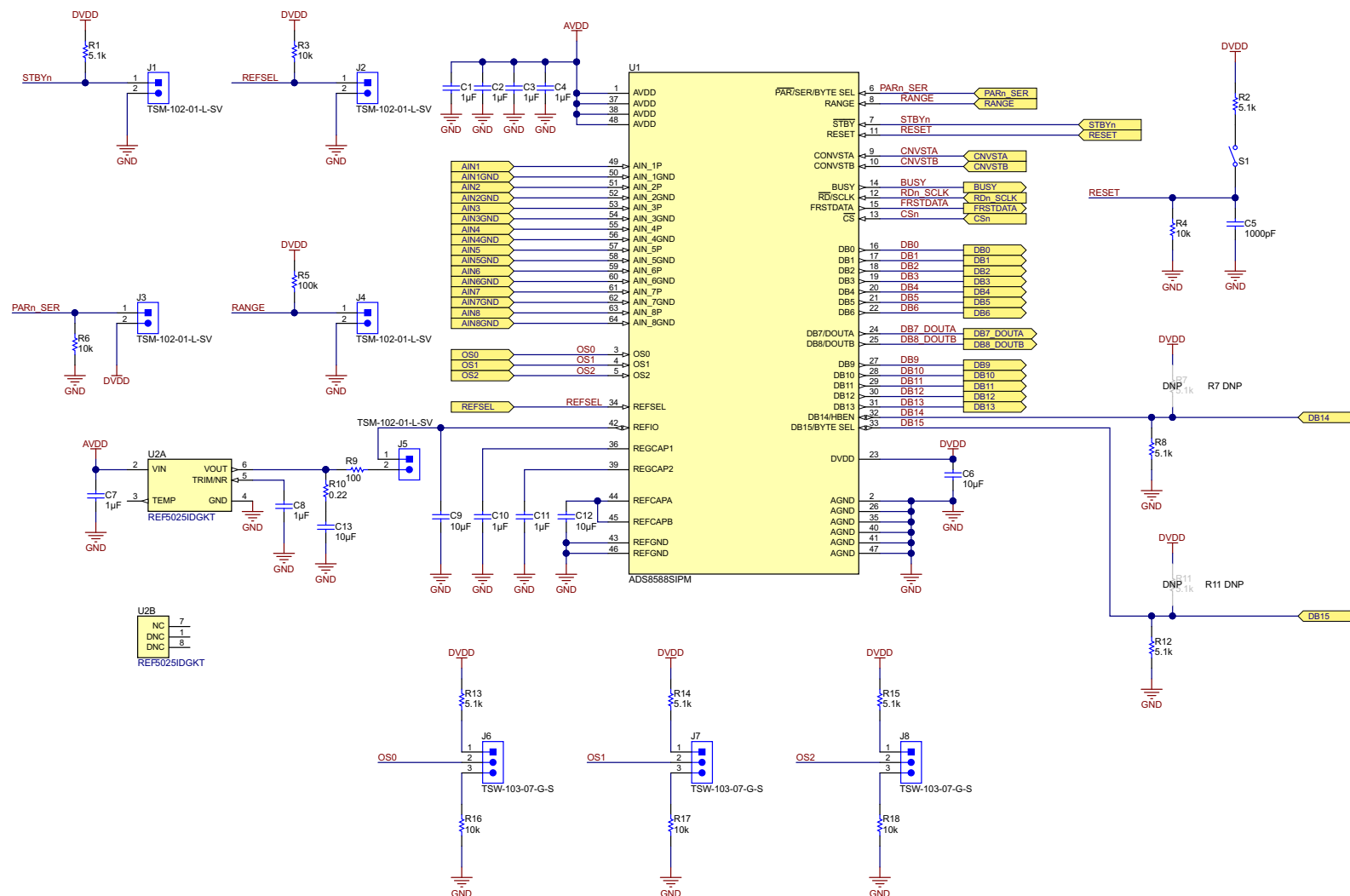
Figure 22. ADS8588EVM-PDK Schematic
