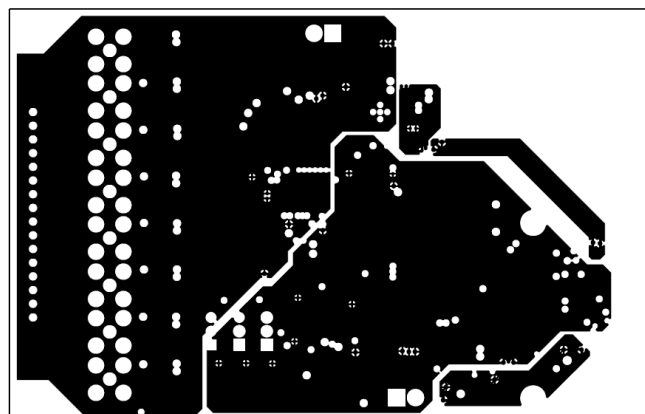
Figure 19. ADS8588S EVM PCB Layer 3: Power Planes
