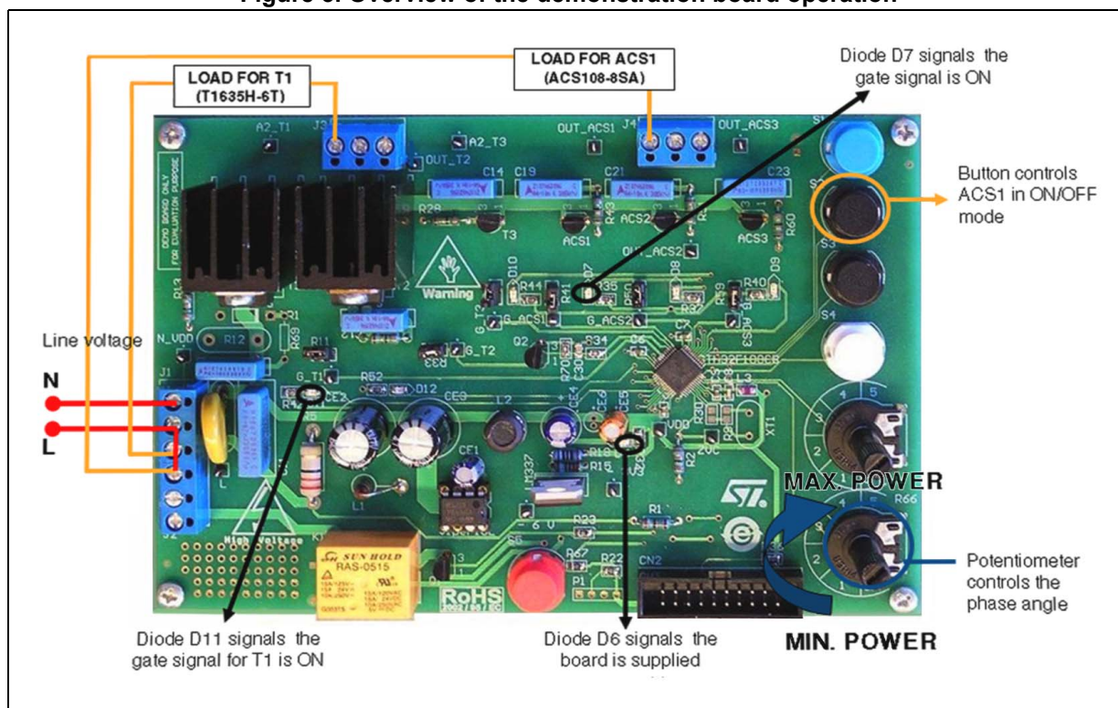
Figure 3. Overview of the demonstration board operation
