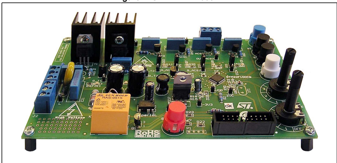
Figure 1. STEVAL-IHT005V2
