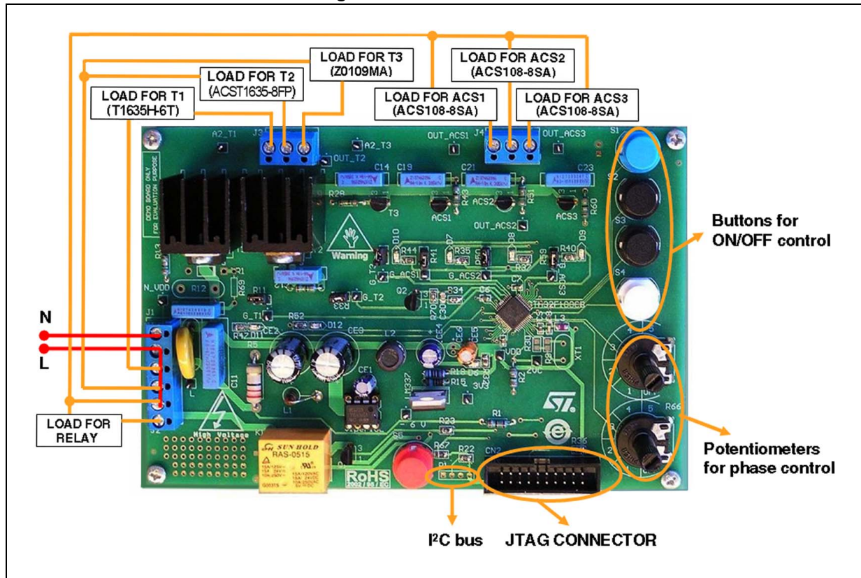
Figure 2. Board connector
