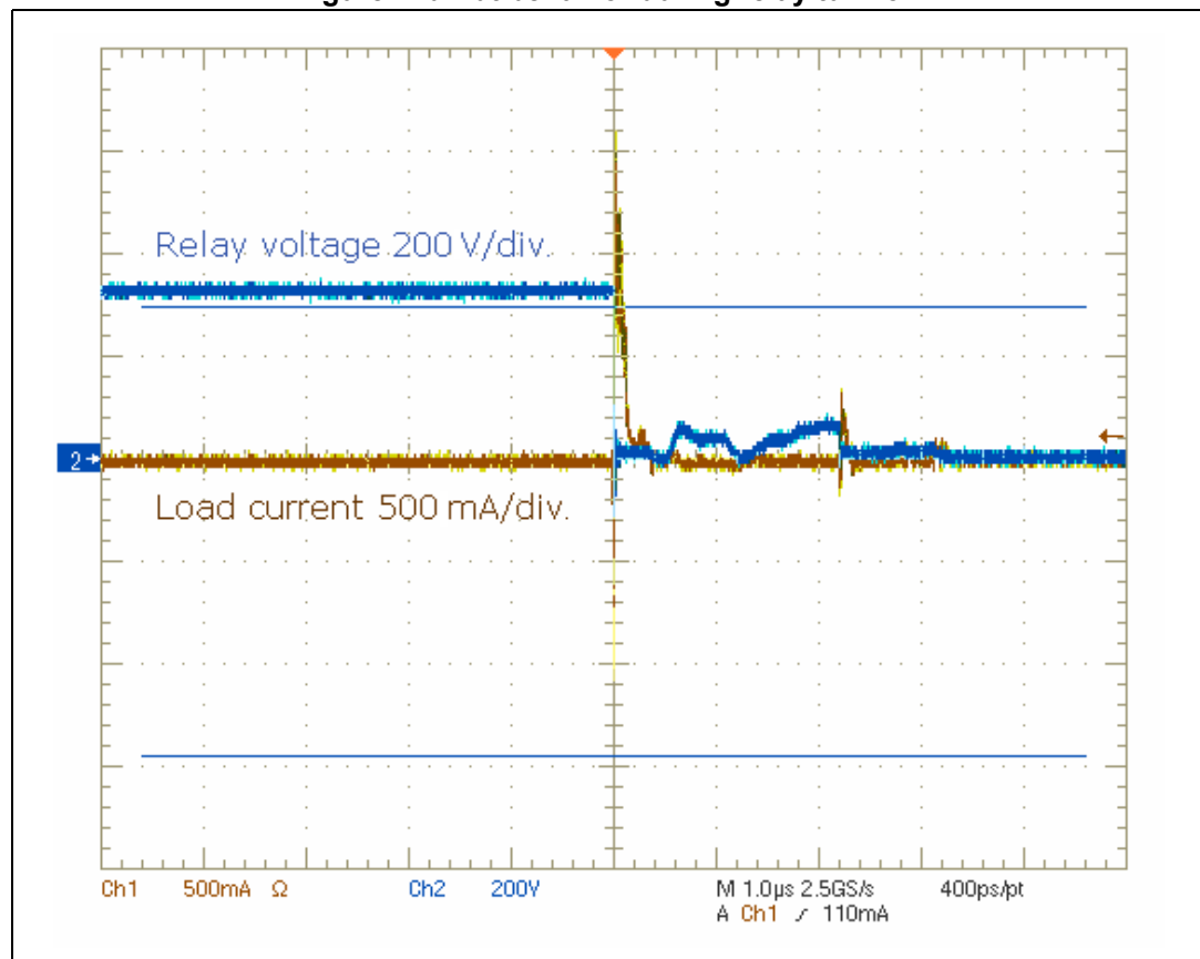
Figure 7. dV/dt behavior during relay turn-off
