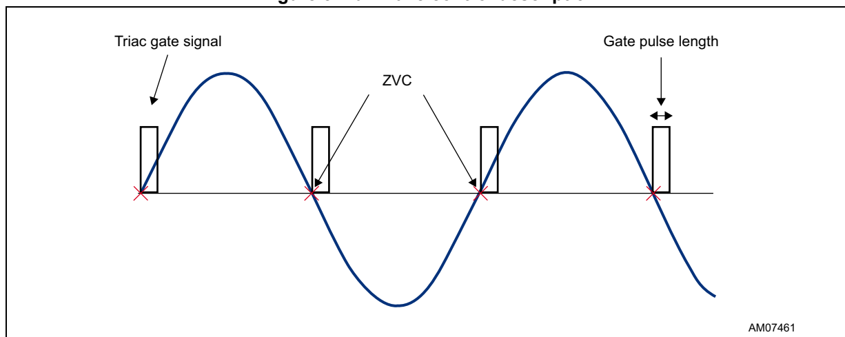
Figure 5. Full wave control description
