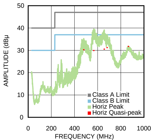
LMZ23603 24Vin to 3.3V @ 3A – EN55022
