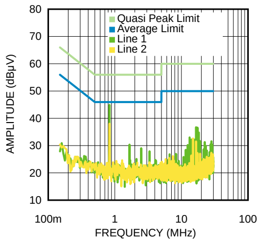
LMZ23605 Conducted EMI
