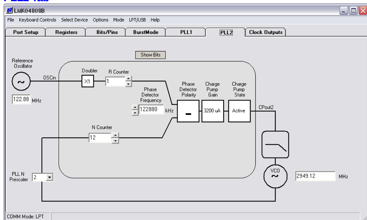
Figure 12: PLL2 tab
