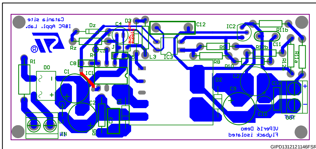
Figure 2: Board layout
