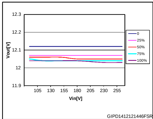
Figure 9: Line regulation
