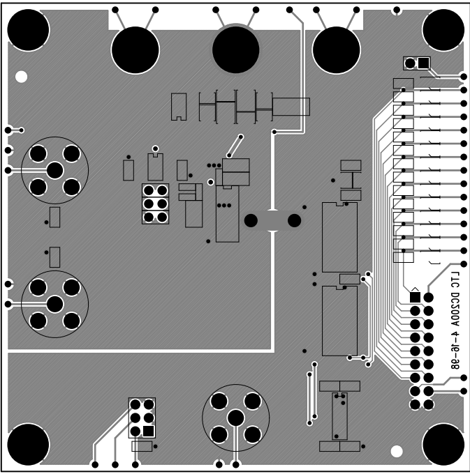
Solder Side
