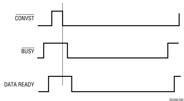
Figure 2. Timing Diagram
