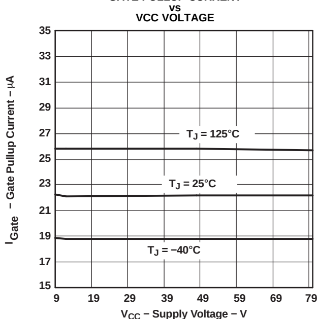
GATE PULLUP CURRENT
