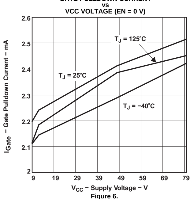
GATE PULLDOWN CURRENT
