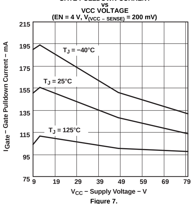
GATE PULLDOWN CURRENT
