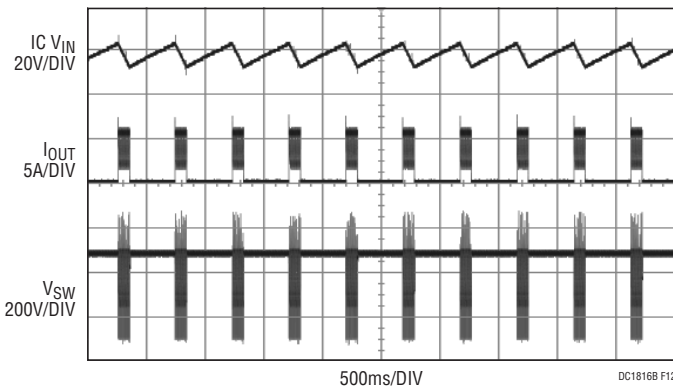
Figure 12. V_{IN} = 277VAC
