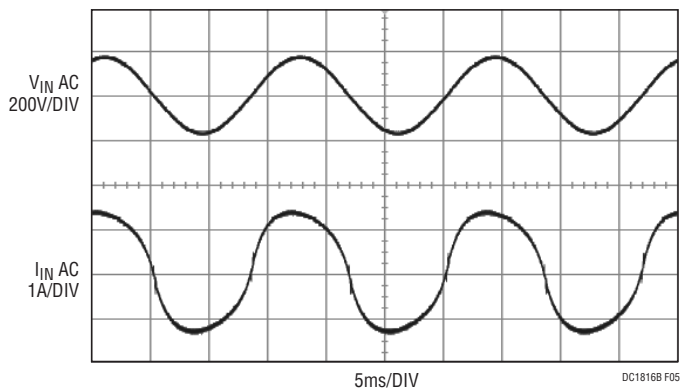
Figure 5. V_{IN} = 120VAC
