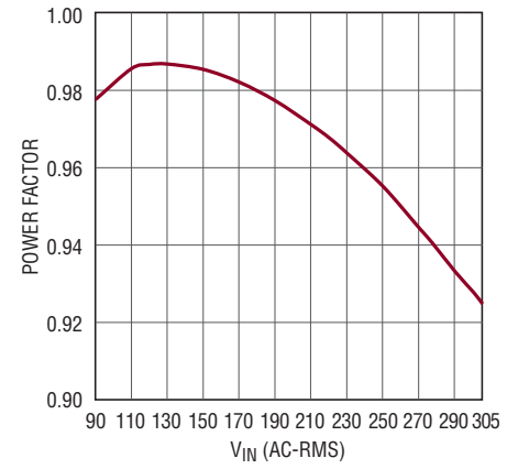
Figure 4. Power Factor vs Input Voltage
