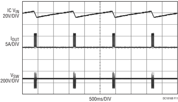
Figure 11. V_{IN} = 120VAC
