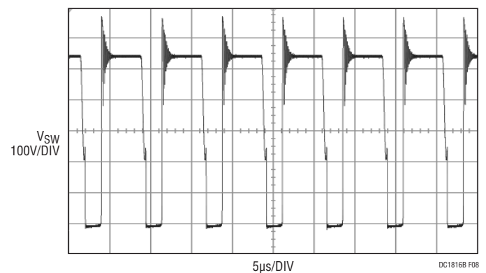
Figure 8. V_{IN} = 277VAC
