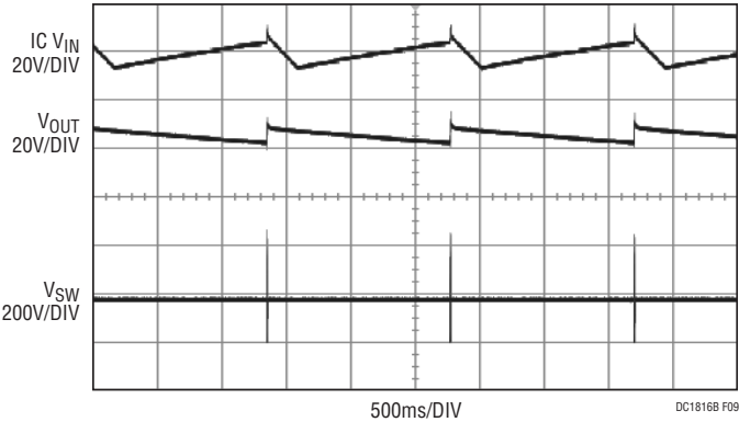
Figure 9. V_{IN} = 120VAC
