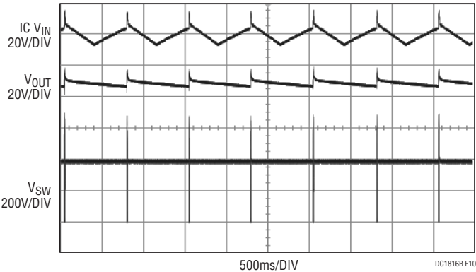
Figure 10. V_{IN} = 277VAC
