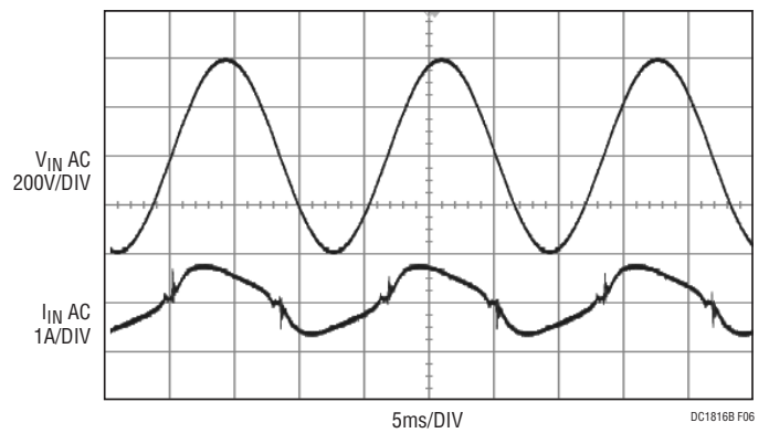
Figure 6. V_{IN} = 277VAC
