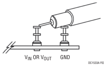
Figure 3. Proper Scope Probe Technique
