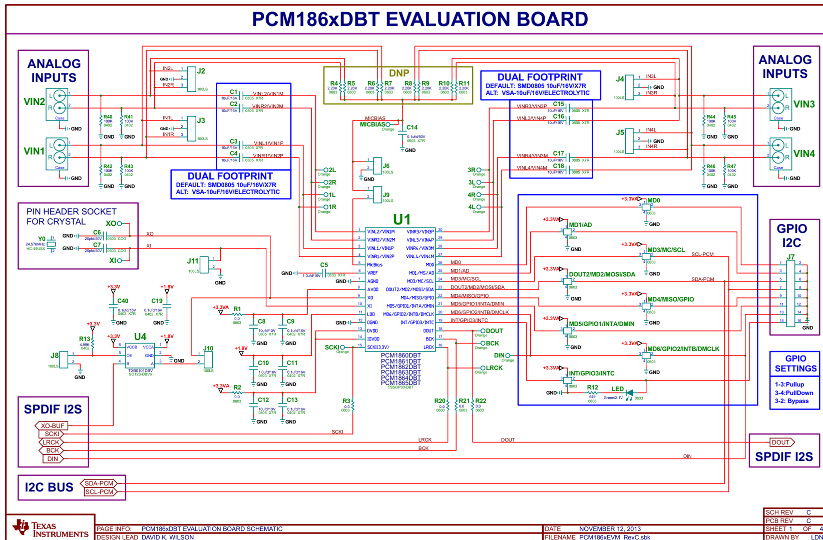
Figure 15. PCM186xEVM Schematic
