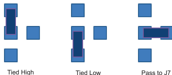
Figure 9. Solder Options
