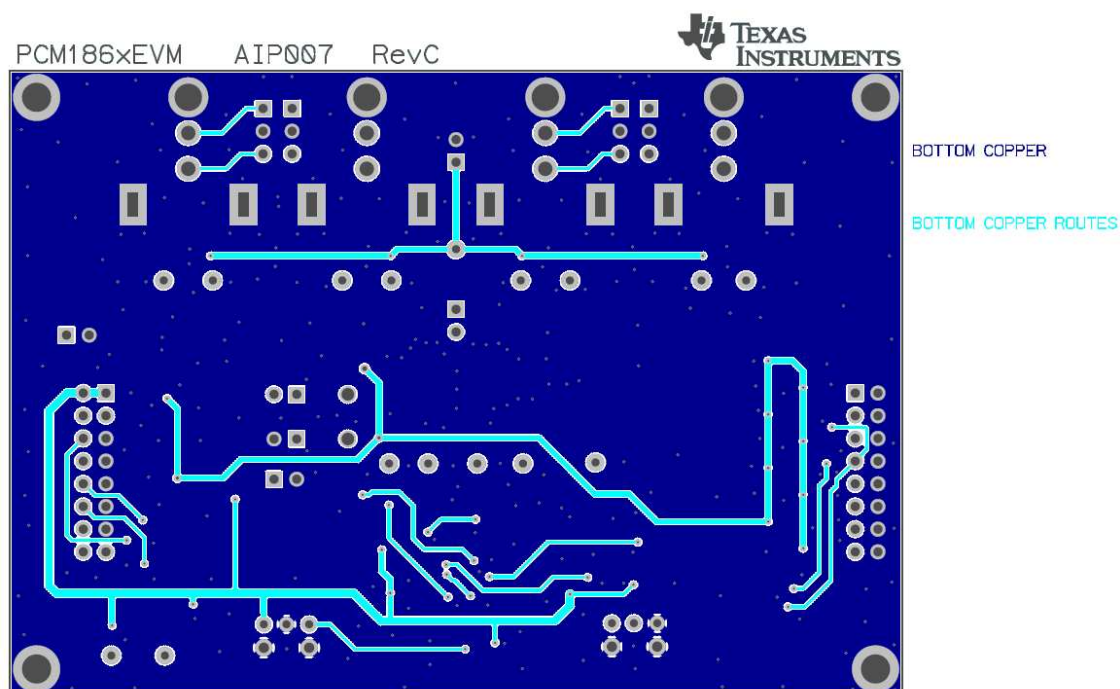
Figure 19. Bottom Copper
