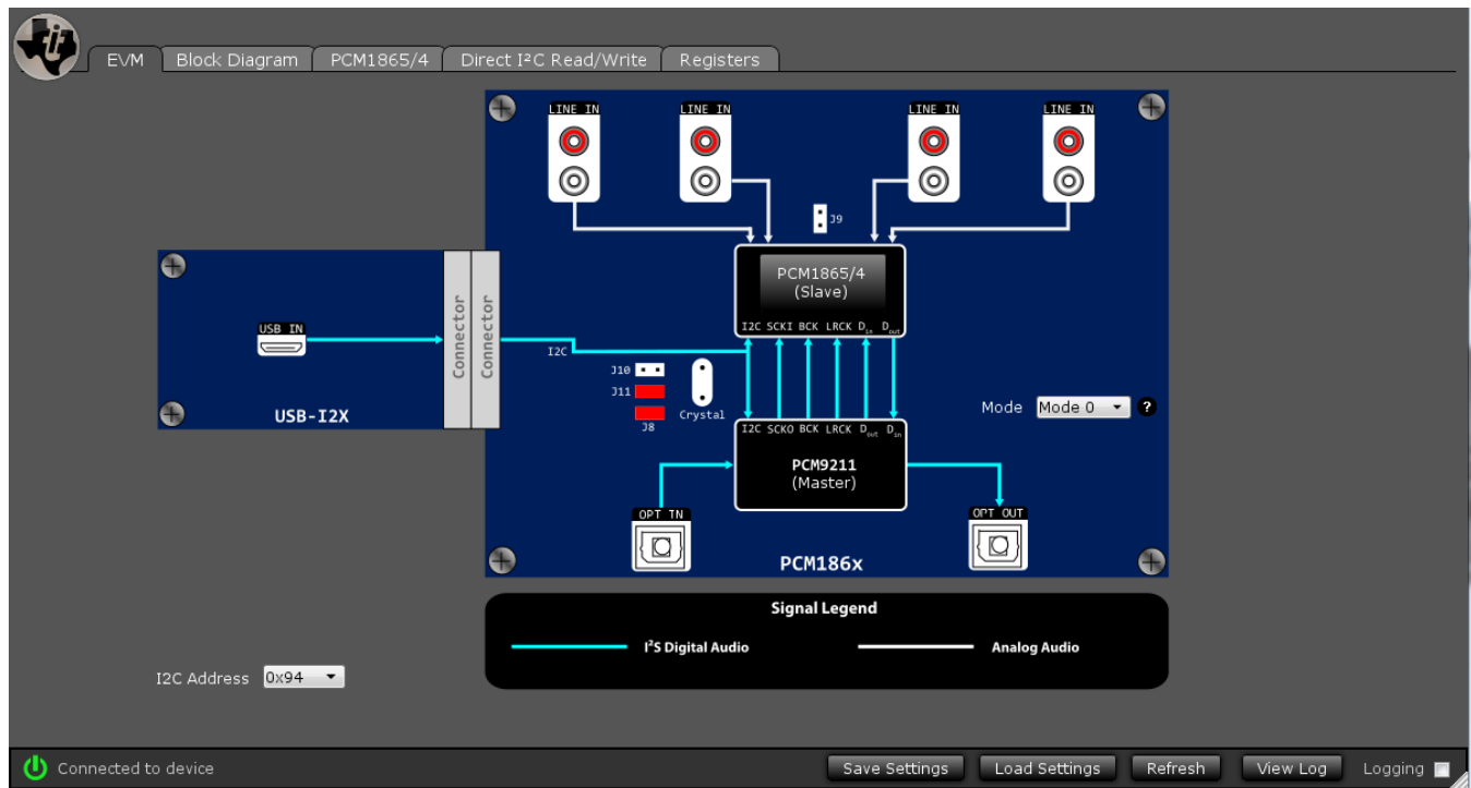
Figure 12. EVM Tab
