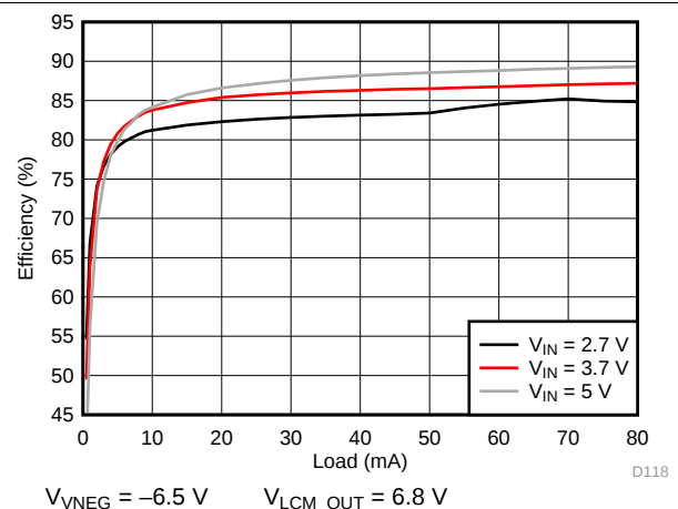
Figure 204. VNEG Efficiency
