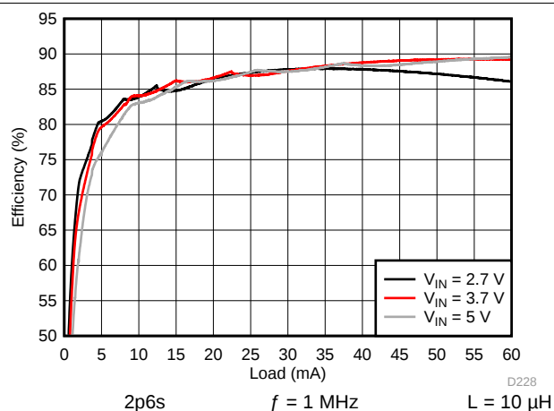
Figure 96. Backlight System Efficiency
