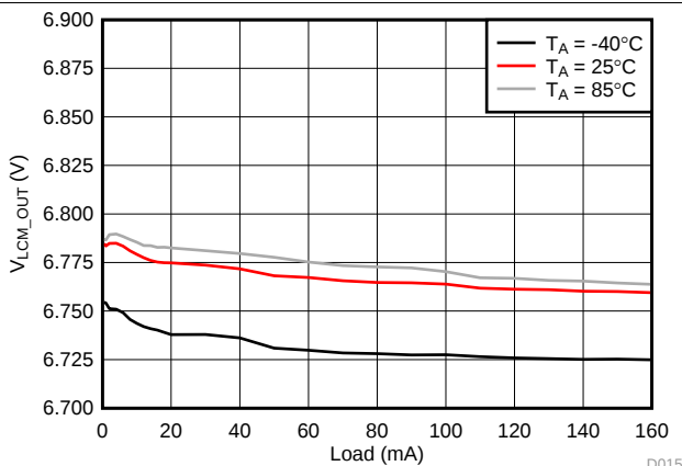
Figure 16. V_{LCM\_OUT} Load Regulation
