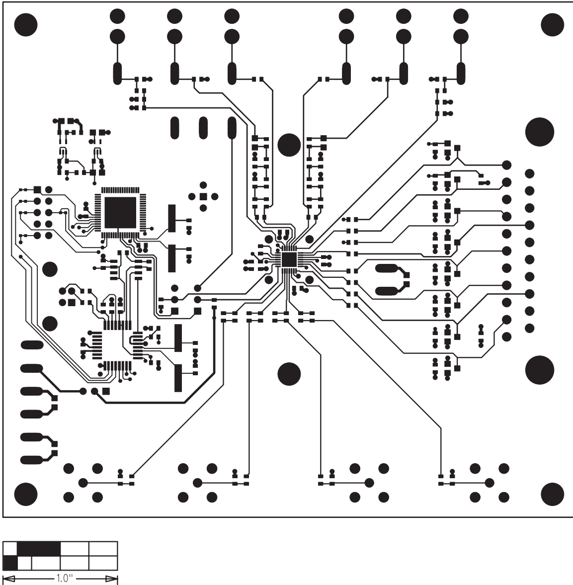
Figure 9. MAX9597 EV Kit Component PCB Layout—Component Side
