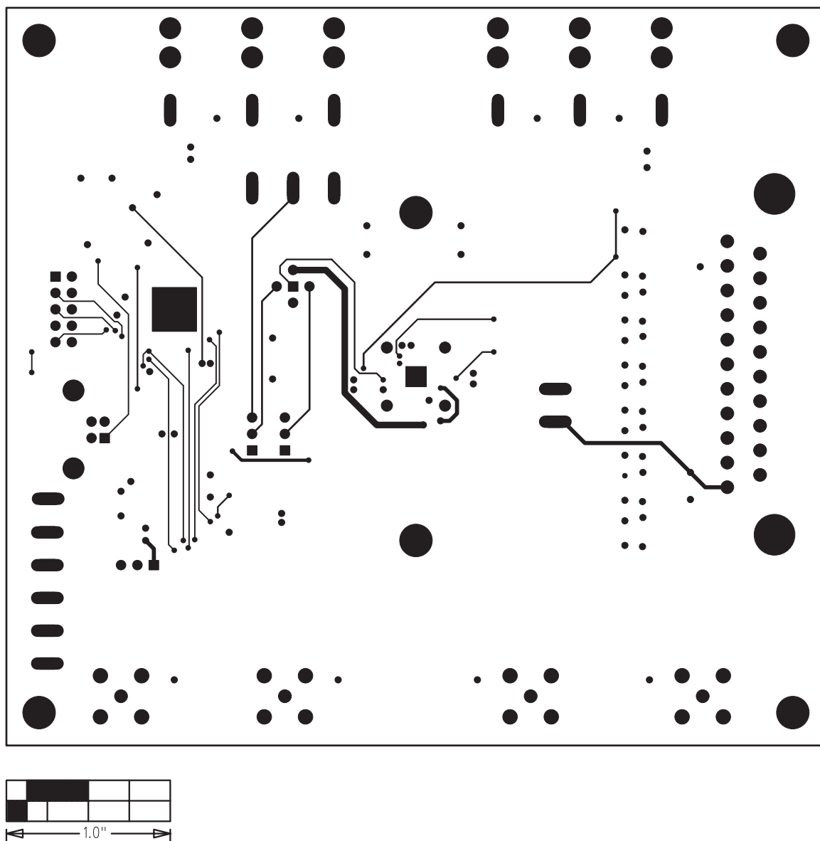
Figure 12. MAX9597 EV Kit PCB Layout—Solder Side
