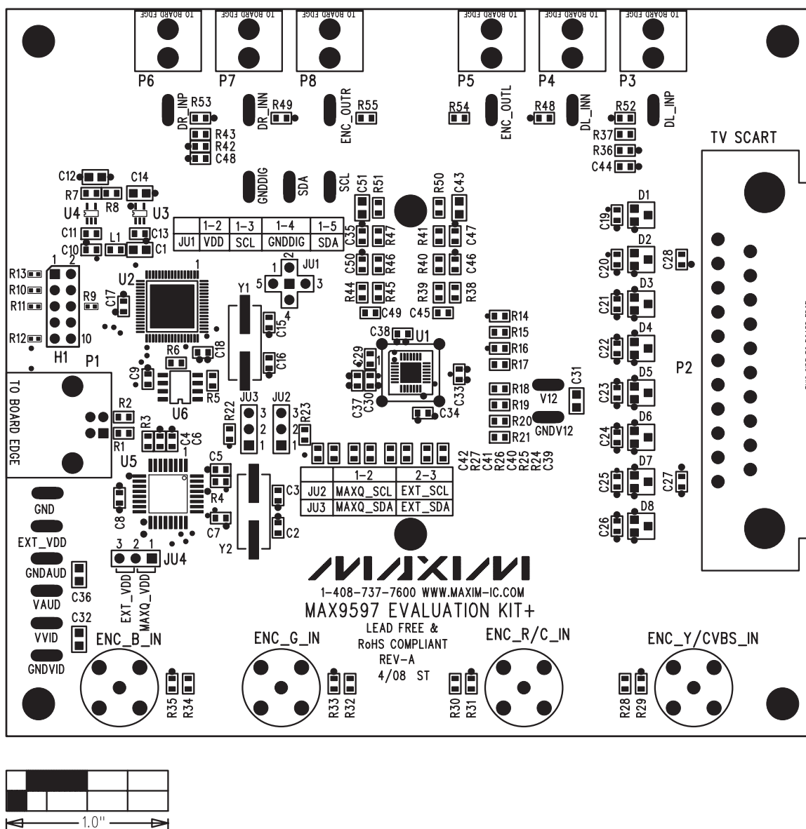
Figure 8. MAX9597 EV Kit Component Placement Guide—Component Side
