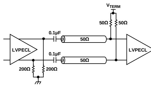
Figure 19. LVPECL AC-Coupled Termination
