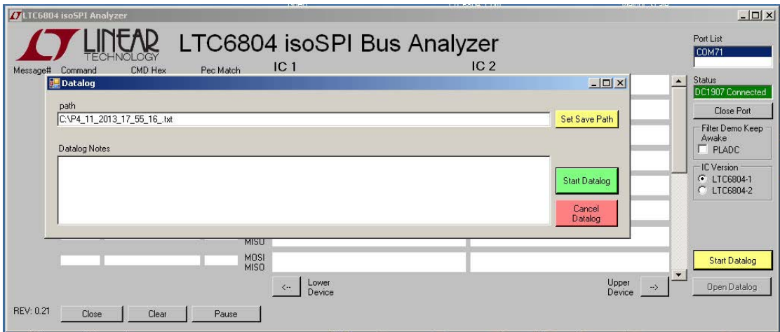
Figure 5. Datalog Dialog
