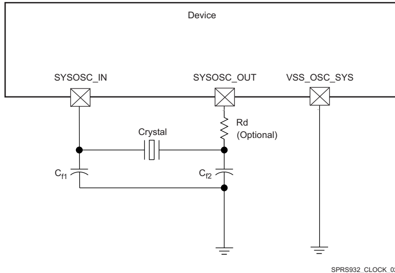
Figure 5-9. Crystal Implementation (1)
