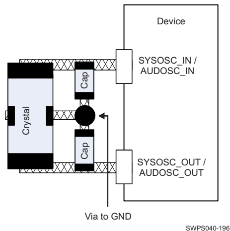
Figure 7-25. SYSOSC and AUDIOOSC PCB requirements
