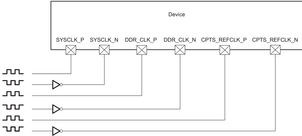
Figure 5-14. LVDS-Compatible Clock Input
