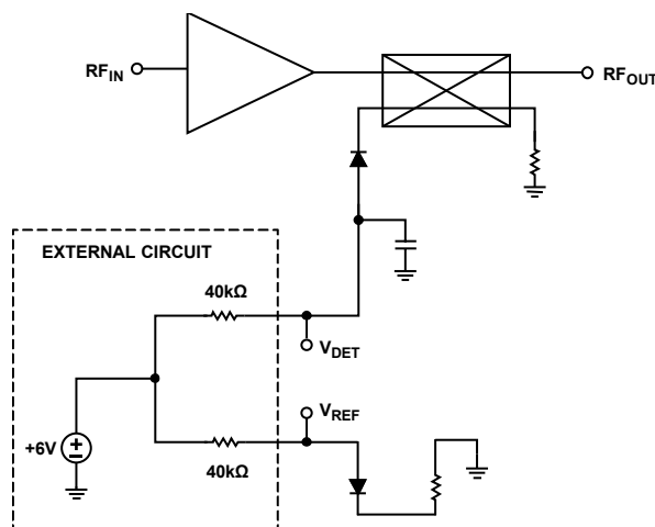
Figure 49. Power Detection Circuit
