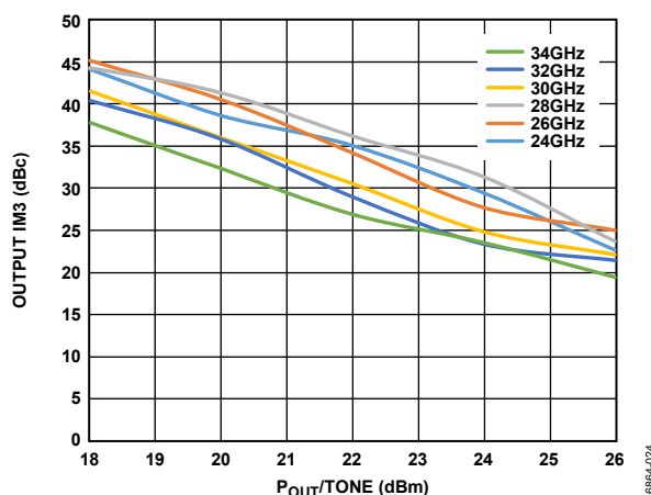
Figure 24. Output IM3 vs. P_{OUT} per Tone, V_{DD} = 5.5 V
