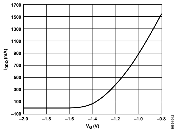
Figure 47. I_{DDQ} vs. Gate Bias Voltage ( V_G ), V_{DK} = 5.5\text{ V} , Representative of a Typical Device
