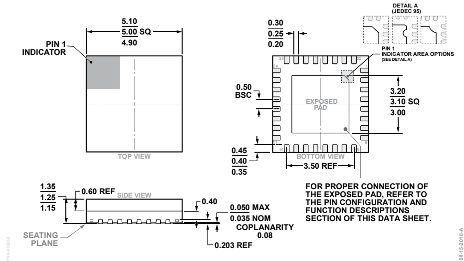
Figure 52. 32-Lead Lead Frame Chip Scale Package [LFCSP_CAV] 5 mm × 5 mm Body and 1.25 mm Package Height (CG-32-2) Dimensions shown in millimeters
