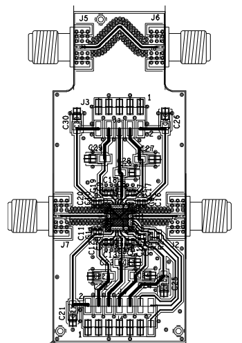
Figure 50. Evaluation PCB
