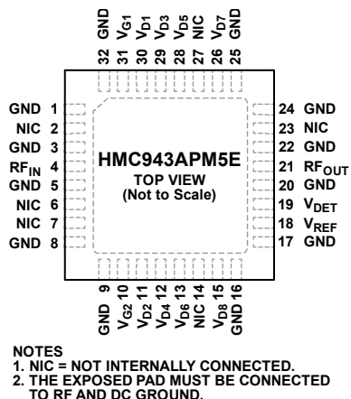
Figure 2. Pin Configuration
