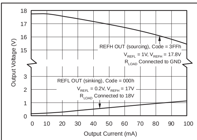
Figure 13. Reference Buffer Output Voltage vs Output Current
