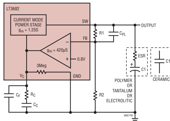
Figure 2. Model for Loop Response
