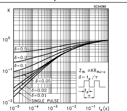
Figure 3. Thermal impedance for DPAK
