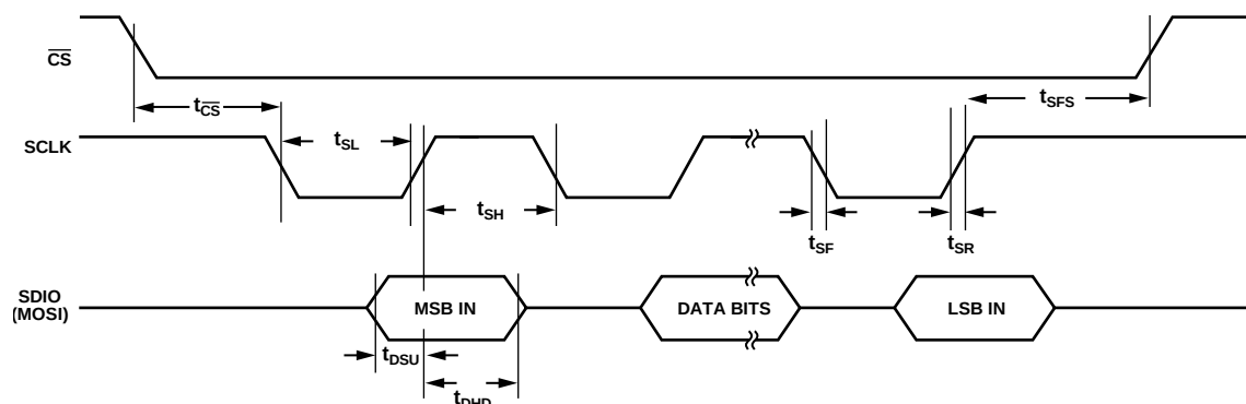
Figure 3. SPI Write Timing Diagram (SPI Master Write to the ADA2200 )
