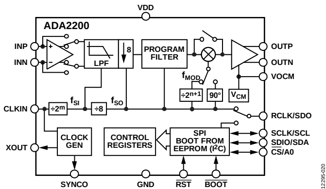
Figure 19. ADA2200 Architecture
