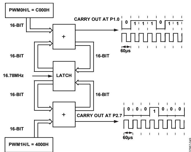
Figure 60. PWM Mode 4
