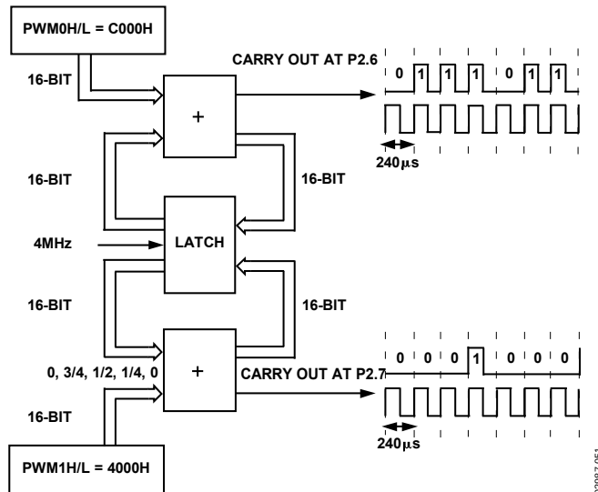
Figure 62. PWM Mode 6
