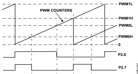
Figure 61. PWM Mode 5
