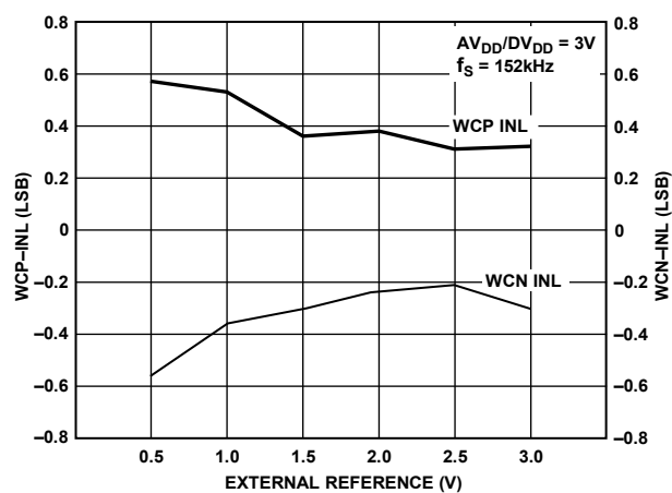
Figure 19. Typical Worst-Case INL Error vs. V_{REF} , V_{DD} = 3V
