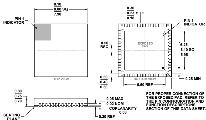
Figure 96. 56-Lead Lead Frame Chip Scale Package [LFCSP]
