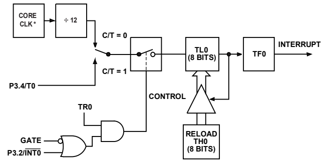
Figure 77. Timer/Counter 0, Mode 2
