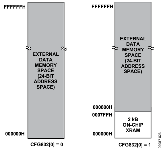
Figure 34. Internal and External XRAM
