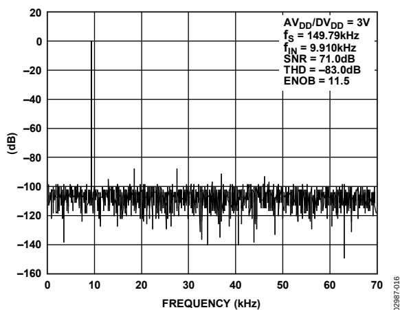
Figure 27. Dynamic Performance at V_{DD} = 3V
