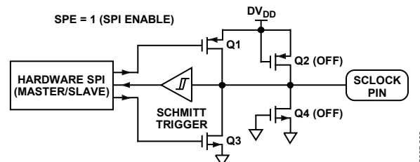
Figure 71. SCLOCK Pin I/O Functional Equivalent in SPI Mode
