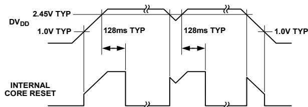
Figure 92. Internal POR Operation
