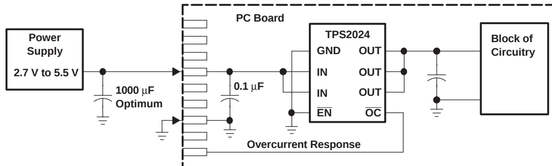
Figure 37. Typical Hot-Plug Implementation
