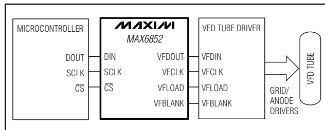
Figure 4. Connection of the MAX6852 to VFD Driver and VFD Tube
