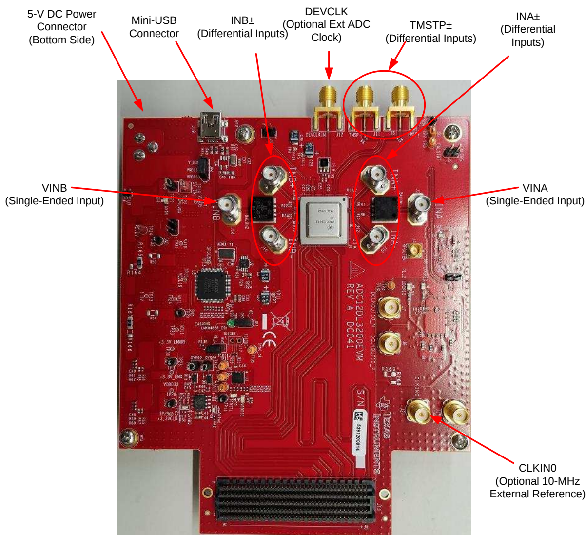
Figure 1-1. EVM Feature Locations
