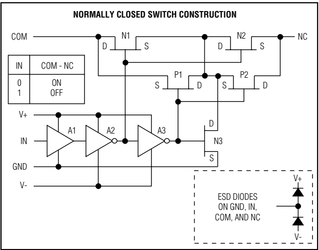
Figure 1. T-Switch Construction
