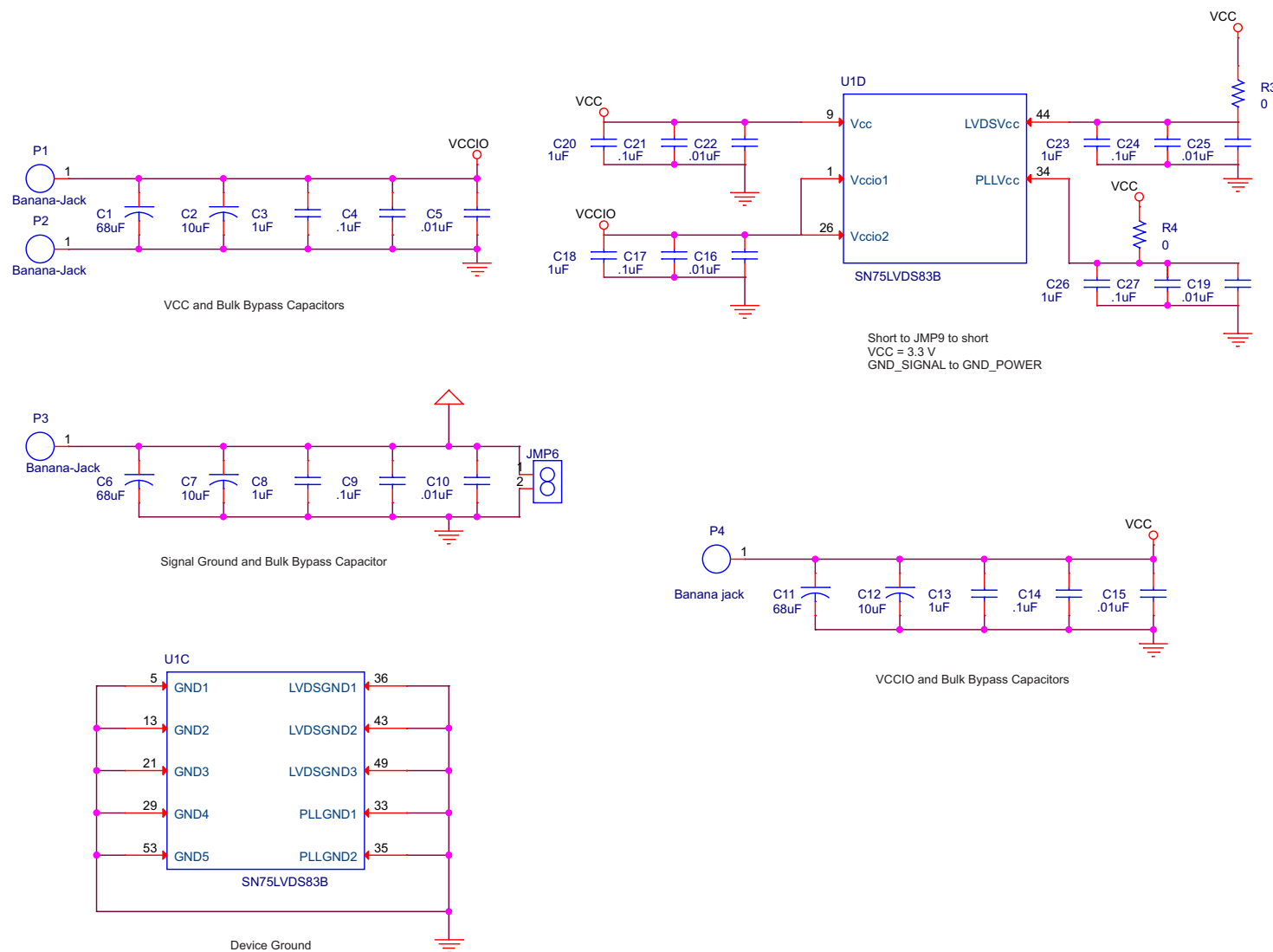
Figure 16. LVDS83BTSSOPEVM Schematics (1/3)
