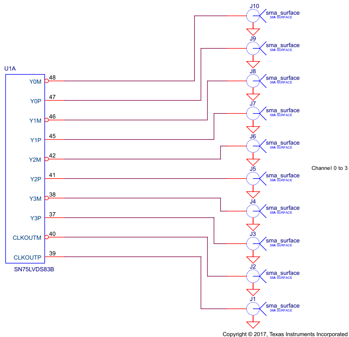
Figure 18. LVDS83BTSSOPEVM Schematic (3/3)
