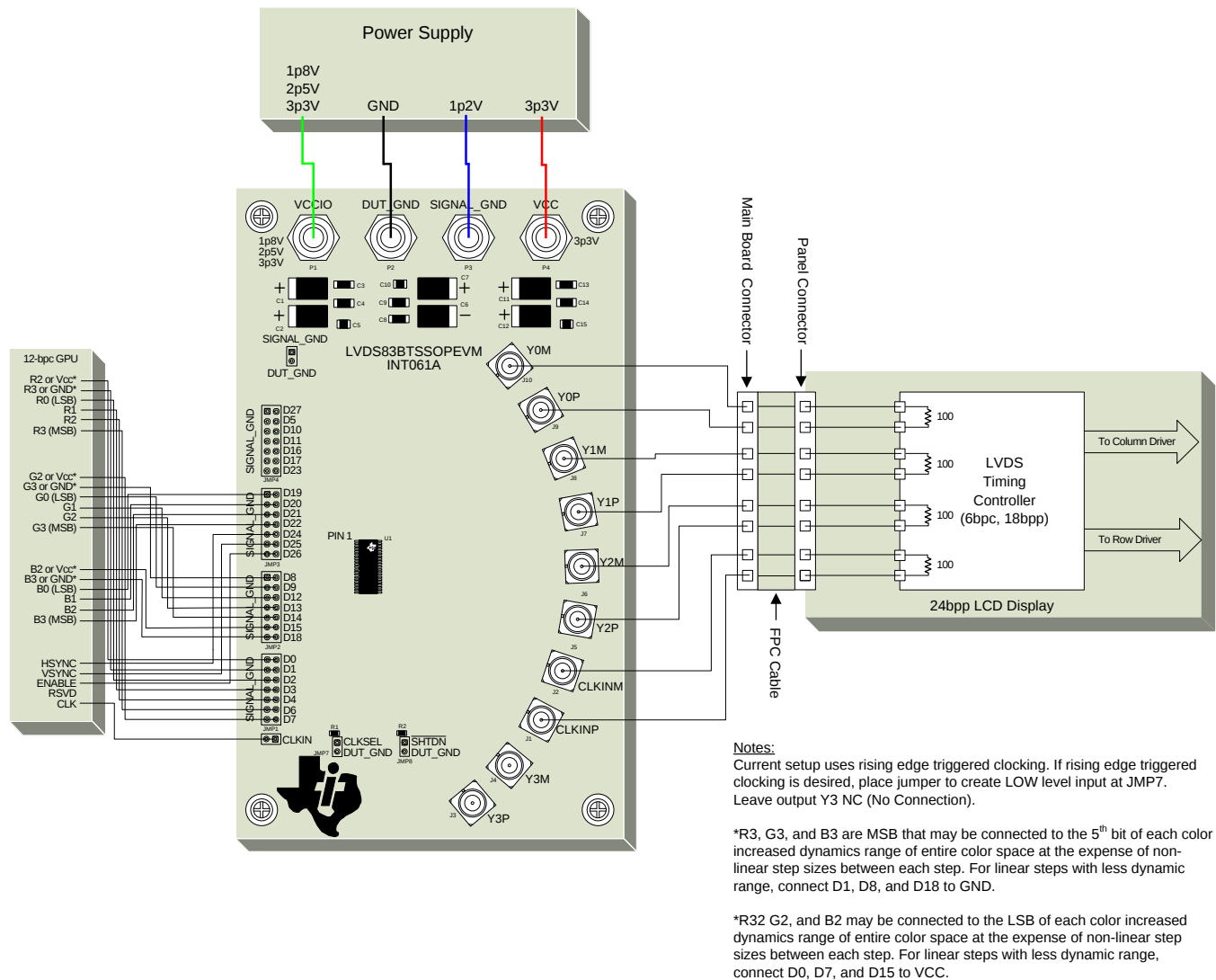
Figure 8. 12-Bit Color Host to 18-Bit LCD Panel Application
