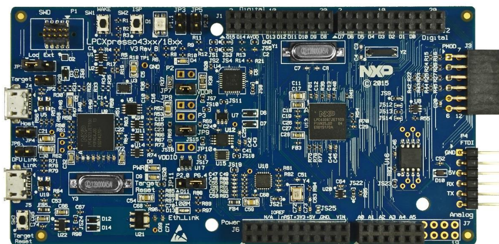
Fig 1. LPCXpresso43xx/18xx
