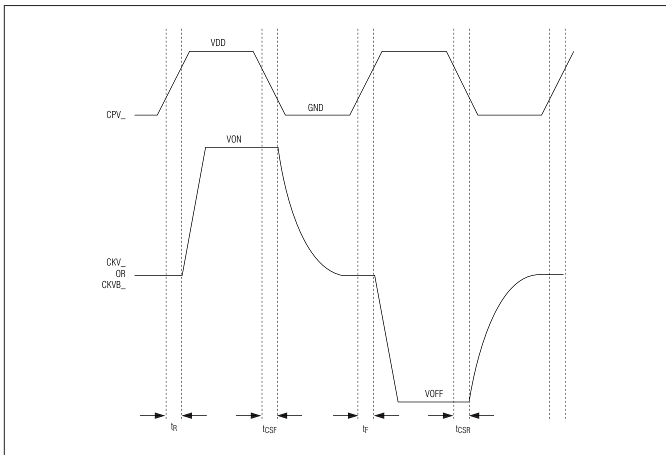
Figure 4. CKV Timing
