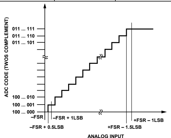
Figure 90. Transfer Function
