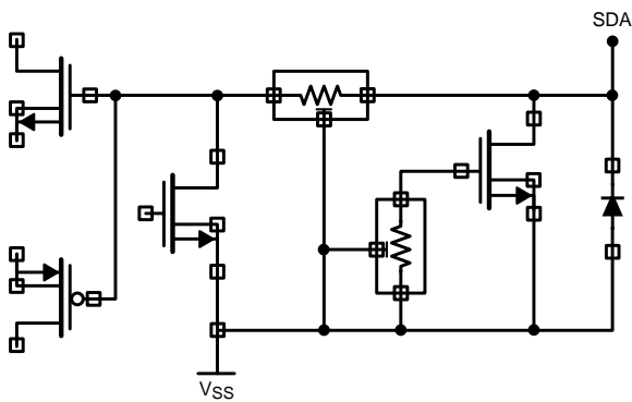
I 2 C DATA CIRCUIT DIAGRAM
