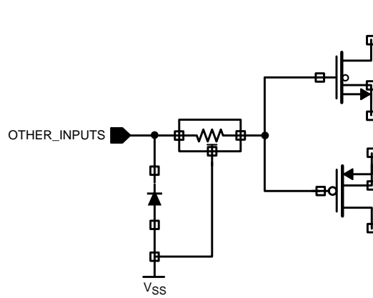
OTHER INPUT CIRCUIT DIAGRAM
