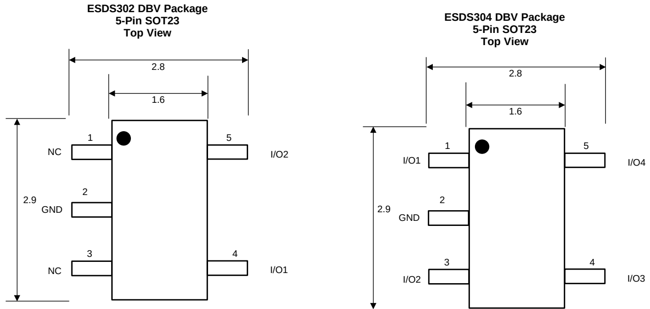
Pin Functions for ESDS302
