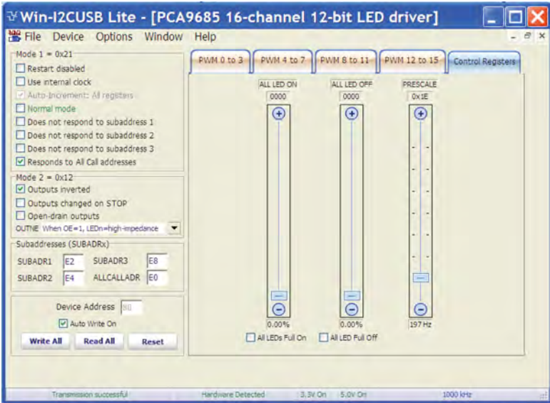
Fig 7. Device configuration screen Control registers
