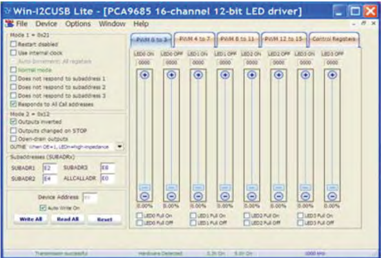
Fig 6. Device configuration screen for PWM0 to PWM3
