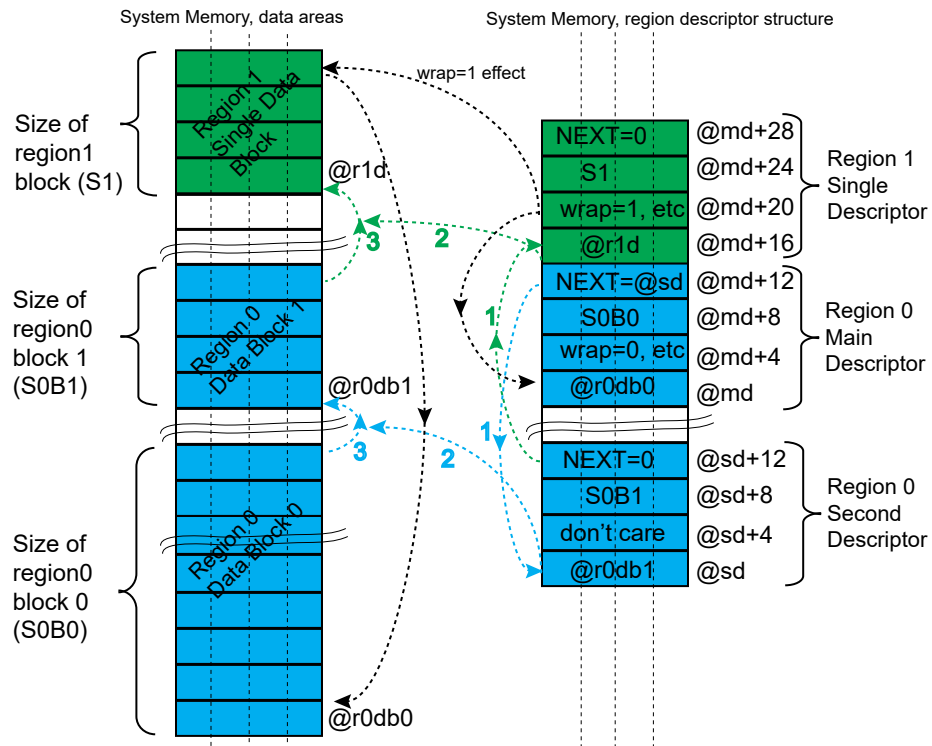
Figure 26-4. Example - Monitoring of 3 Memory Data Blocks (Defined as 2 Regions)
