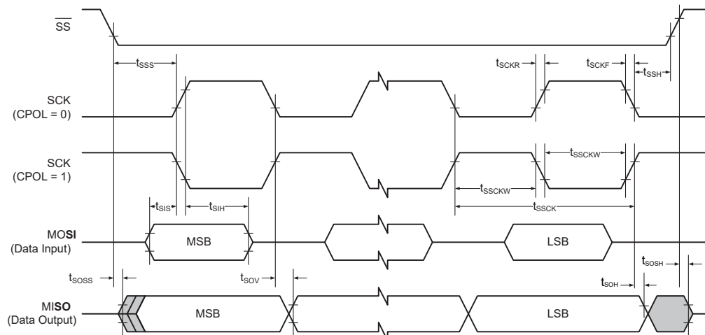
Figure 54-9. SPI Timing Requirements in Slave Mode
