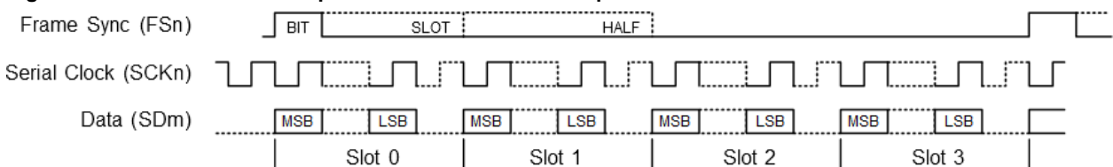
Figure 51-6. TDM Format Reception and Transmission Sequence
