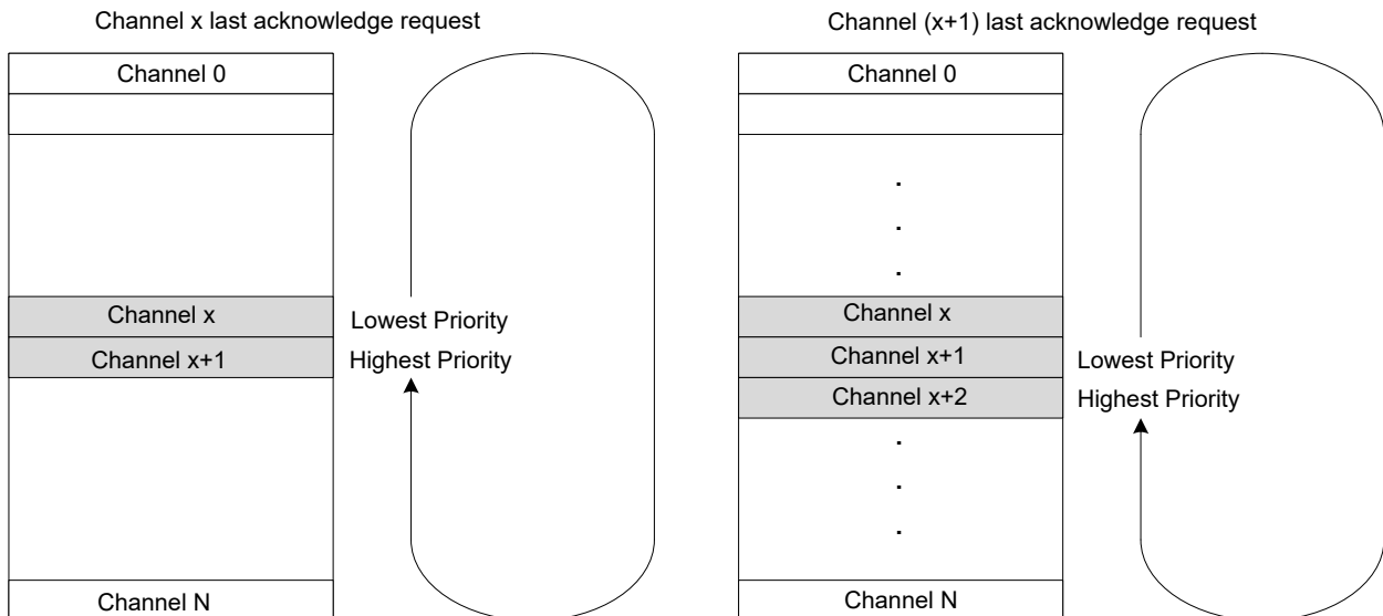
Figure 31-4. Round-Robin Scheduling
