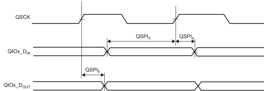
Figure 54-12. QSPI SDR Master Mode 2
