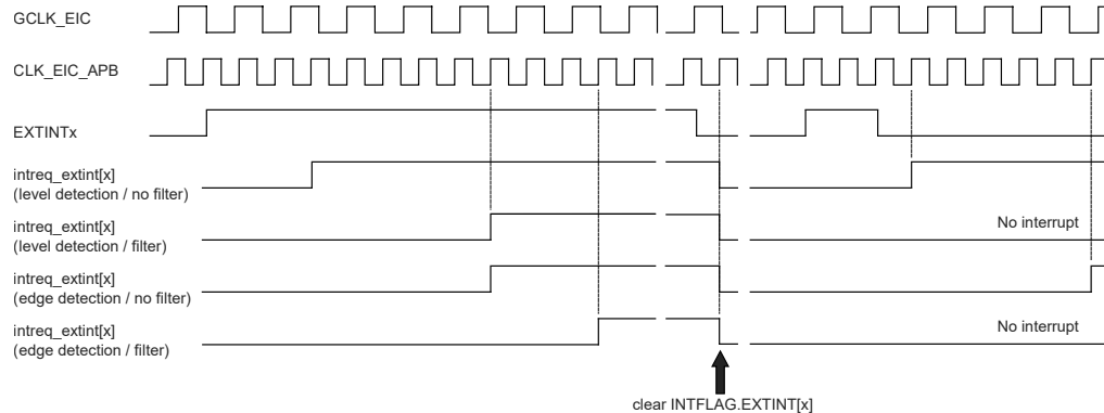
Figure 23-2. Interrupt Detection Latency by modes (Rising Edge)
