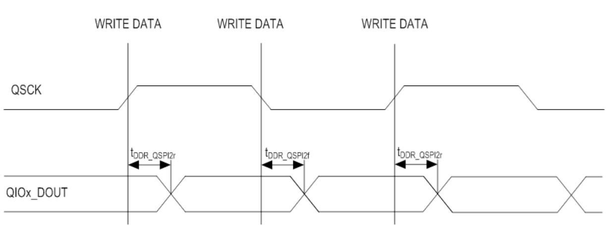
Figure 54-15. QSPI DDR Mode 0 WRITE
