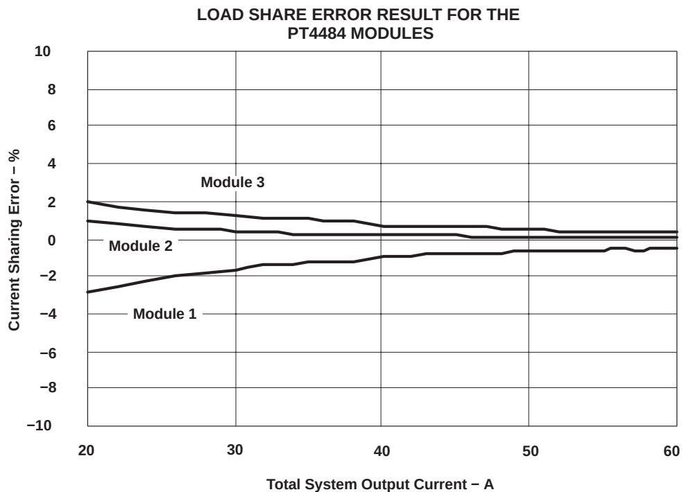
Figure 15. Resultant Load Current Sharing Accuracy, as Measured Across Shunts from the Output of Each Module.
