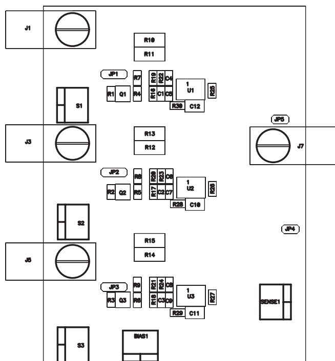
Figure 5. Top View
