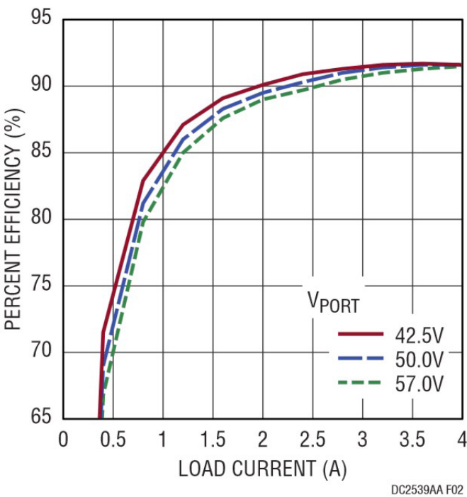
Figure 2. Efficiency (End-to-End)
