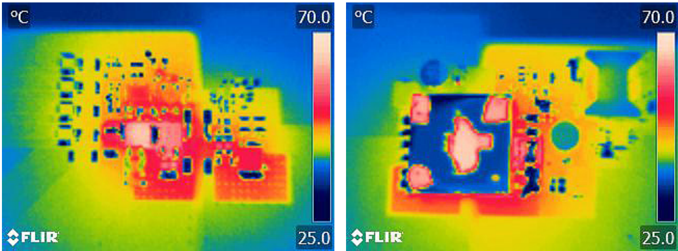
Top Side Bottom Side Figure 1. Thermal Pictures (Conditions: V_{PORT} = 57V , V_{OUT} = 12V , I_{OUT} = 3.9A )
