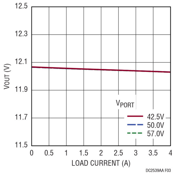
Figure 3. Load Regulation
