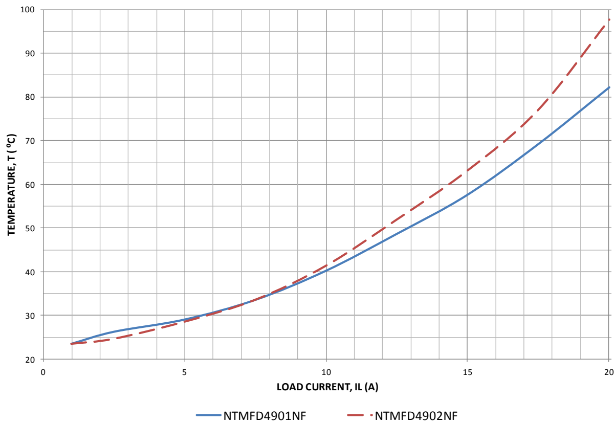
Figure 6: Comparison of Device Temperatures
