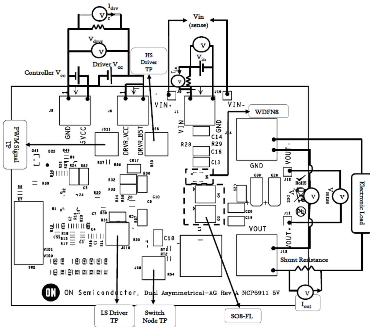
Figure 3: Schematic of the Test Setup
