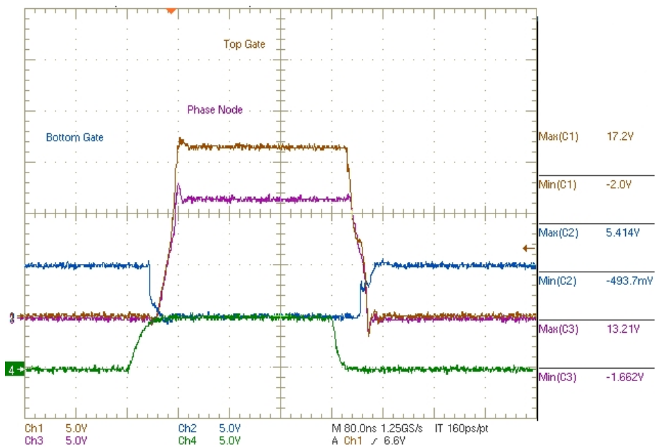
Figure 9: PWM Signal at G1 for I_{out} = 0A
