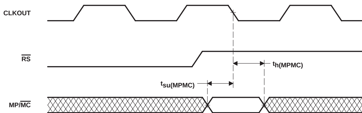
Figure 5-17. \text{MP}/\overline{\text{MC}} Timing
