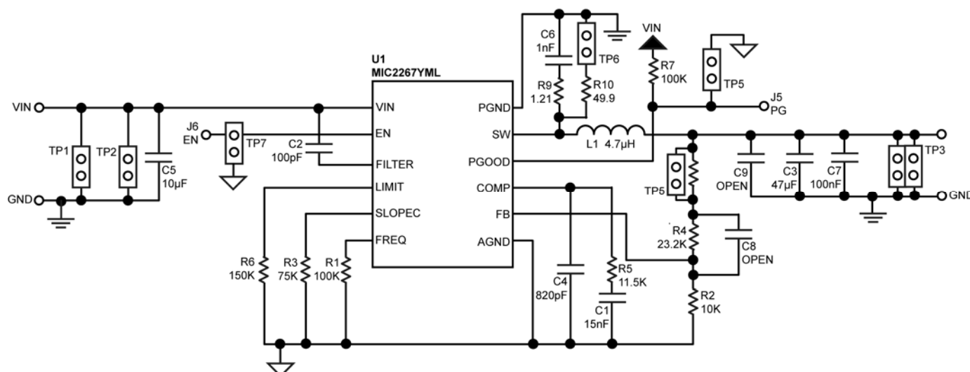
MIC2267 Typical Application Circuit
